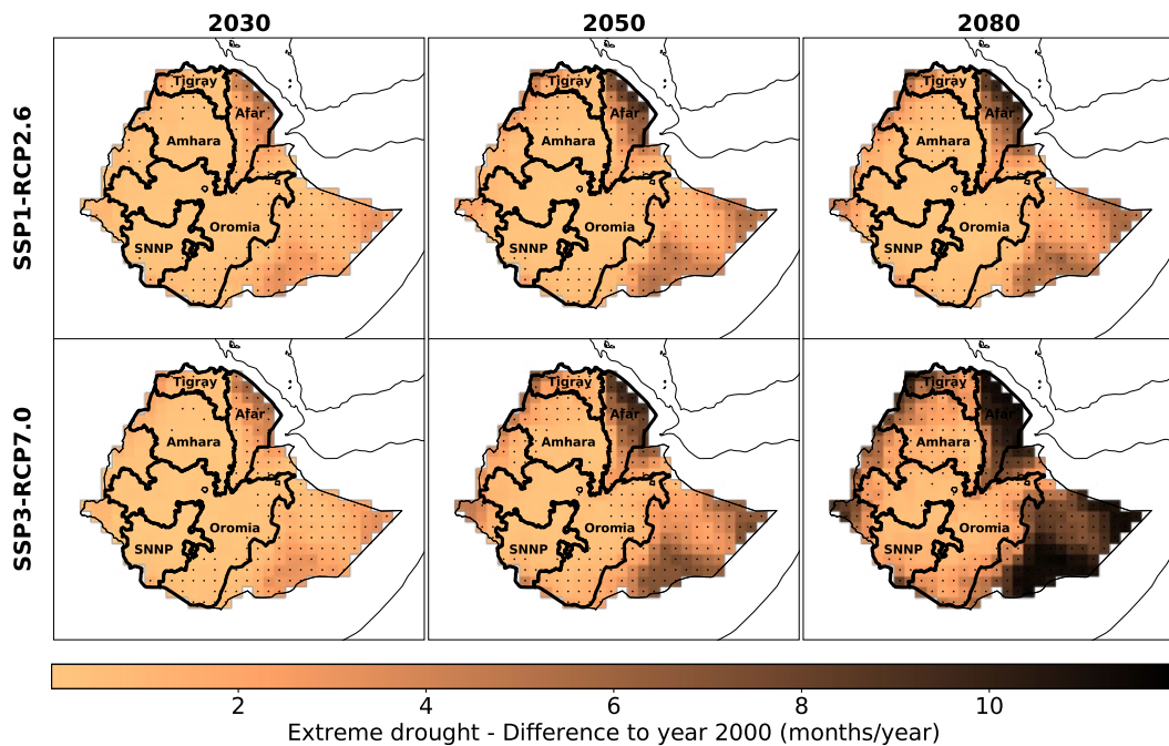
Figure 12: Projected changes in extremely dry months across Ethiopia in 2030, 2050 and 2080 under two different trajectories compared to 2000. Dots indicate that at least 9 out of 10 models agree on the sign of change.
