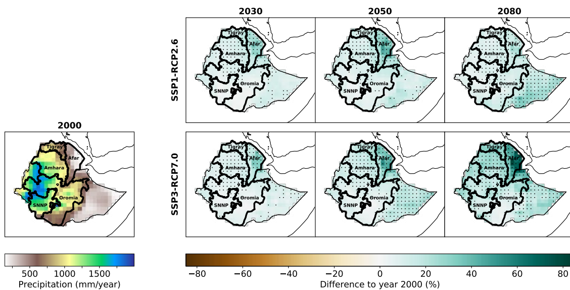
Figure 3: Projected changes of annual precipitation sums across Ethiopia in 2030, 2050 and 2080 under two different trajectories compared to 2000. Dots indicate that at least 9 out of 10 models agree on the sign of change.
